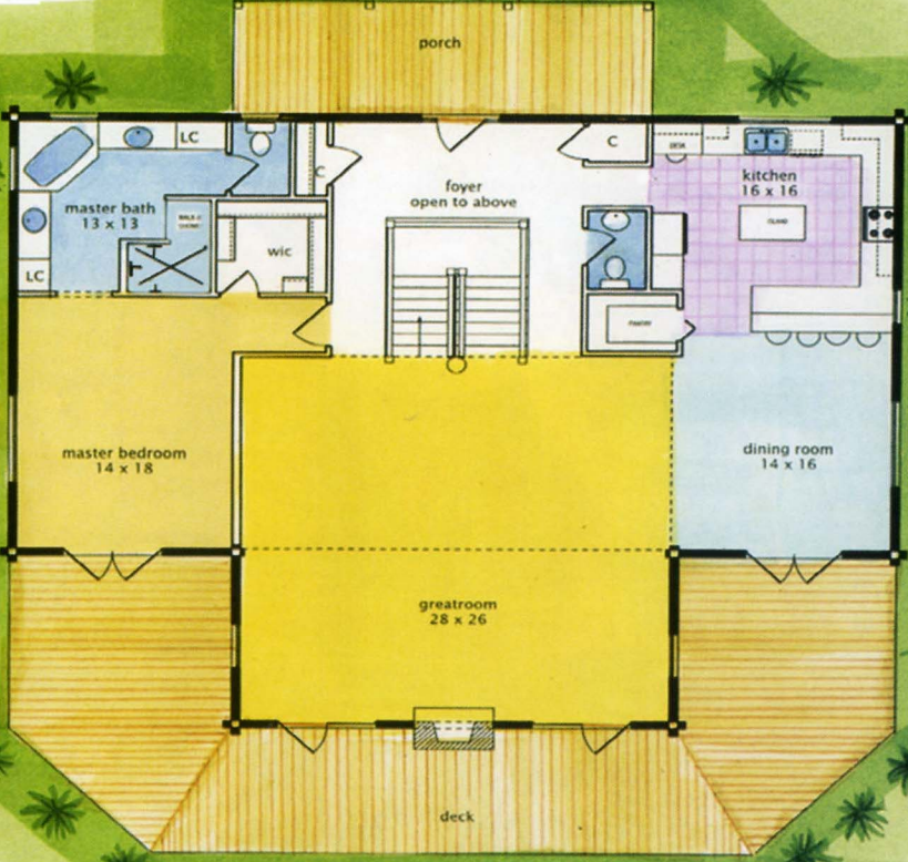
Georgia -- 1st. floor plan
