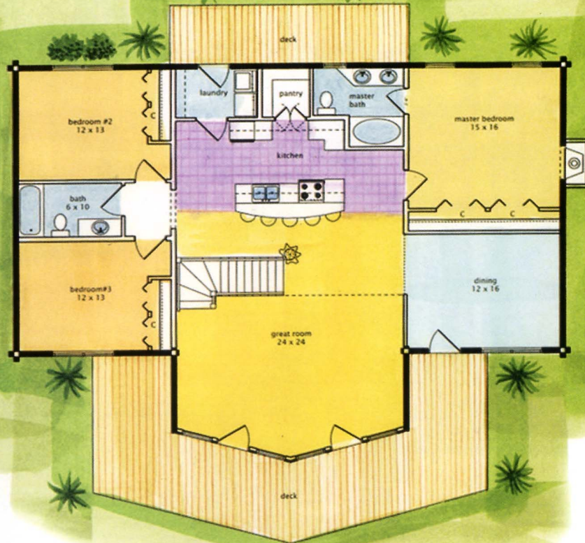
tennessee-- 1st. floor plan
